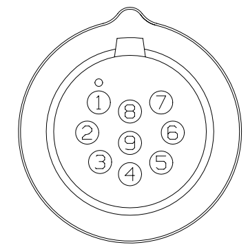
CONTACT END VIEW
